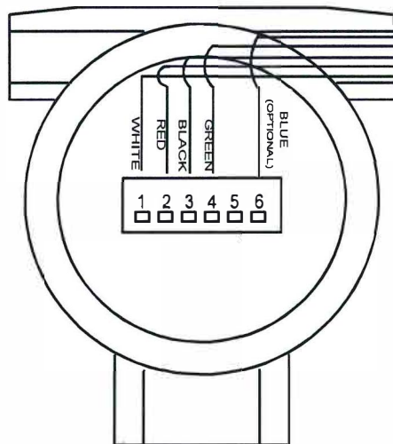
FLOW TRANSDUCER
